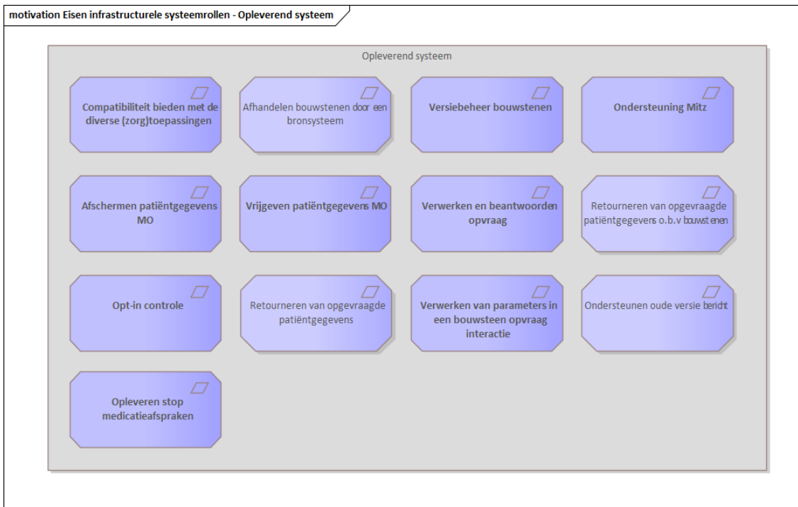
Figure 4 : Eisen infrastructurele systeemrollen - Opleverend systeem
